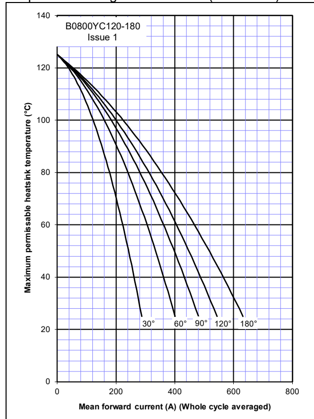
Figure 10 – On-state current vs. Heatsink temperature - Single Side Cooled (Sine wave)
