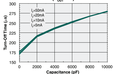
Turn-Off Time vs. Capacitance ( V_{OUT}=1V )
