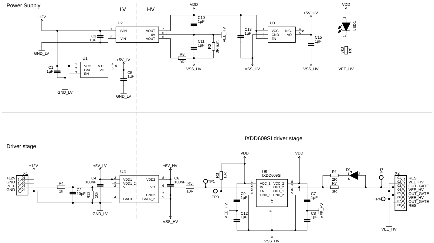
Figure 3. IXDD609SI evaluation board schematics
