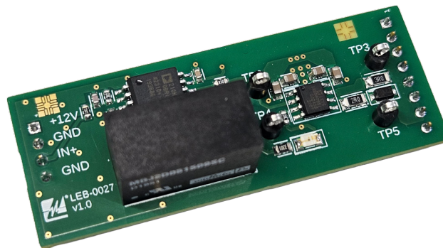
Figure 1. IXDD609SI gate driver evaluation board
