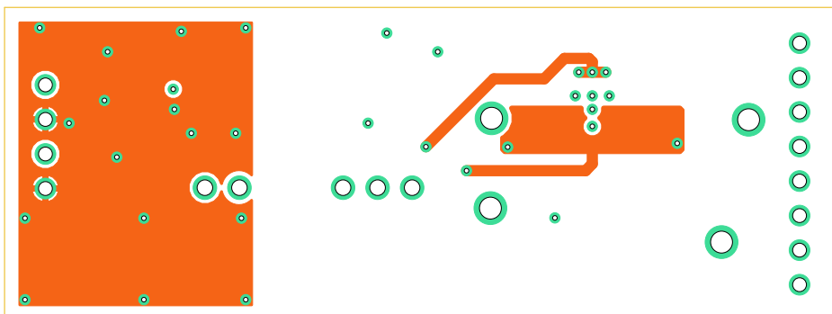
Figure 6. PCB layer 3
