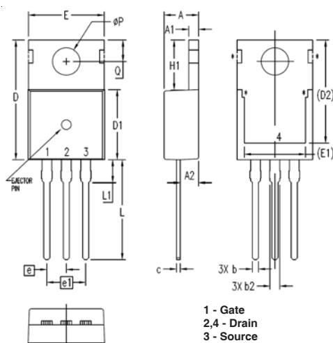
TO-220 Outline
