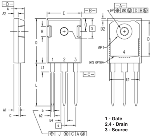
TO-247 Outline
