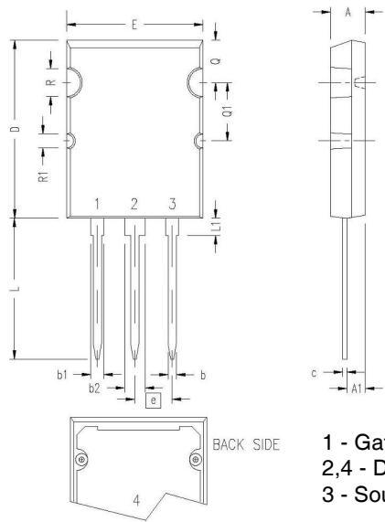
PLUS264™ (IXFB) Outline
