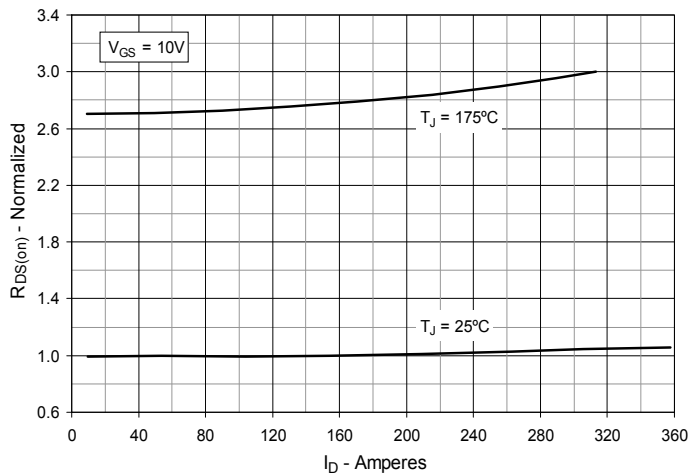
Fig. 5. R_{DS(on)} Normalized to I_D = 120\text{A} Value vs. Drain Current
