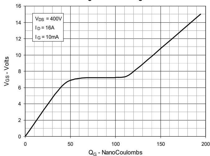
Fig. 10. Gate Charge
