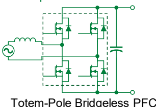
Totem-Pole Bridgeless PFC
