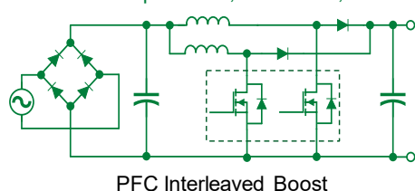
PFC Interleaved Boost
