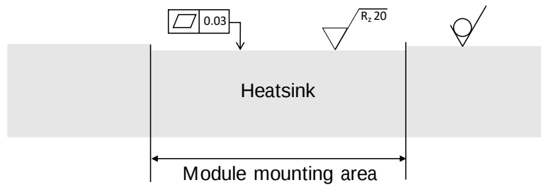
Figure 3. Heat Sink's Surface Requirements to Mount Power Modules
