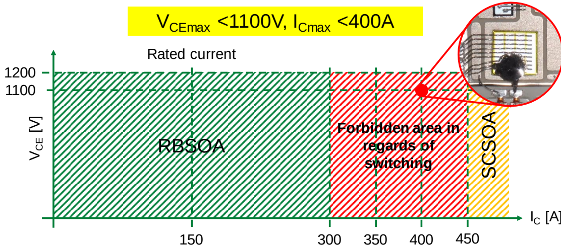
Figure 8. Locating the point of turn-off
