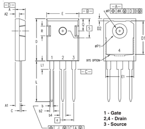
TO-247 Outline
