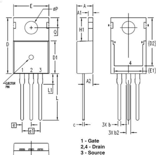
TO-220 Outline
