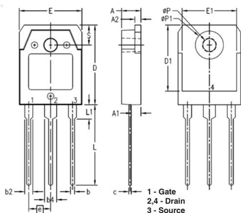
TO-3P Outline
