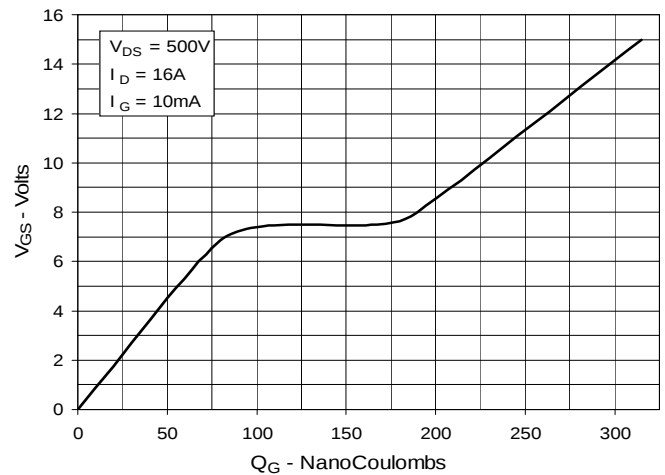
Fig. 10. Gate Charge
