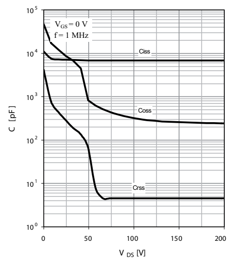
Fig. 9 Typ. capacitances
