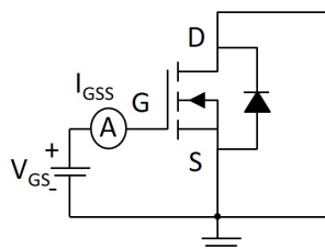
Figure 9. Circuit Diagram to Measure Gate Leakage Current
