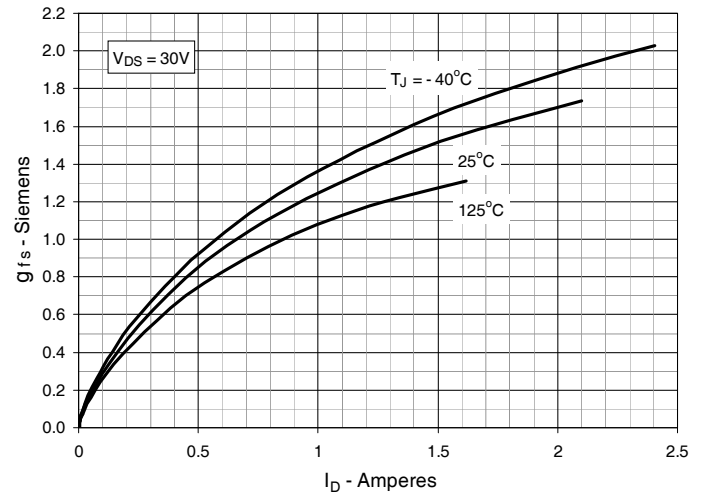
Fig. 10. Transconductance
