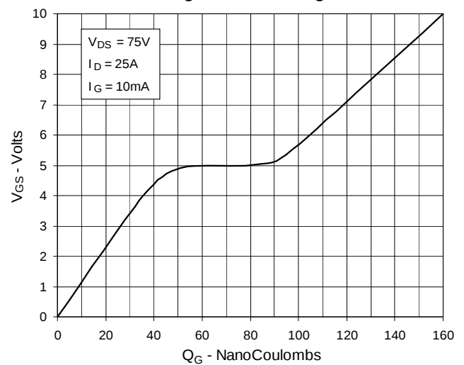
Fig. 10. Gate Charge
