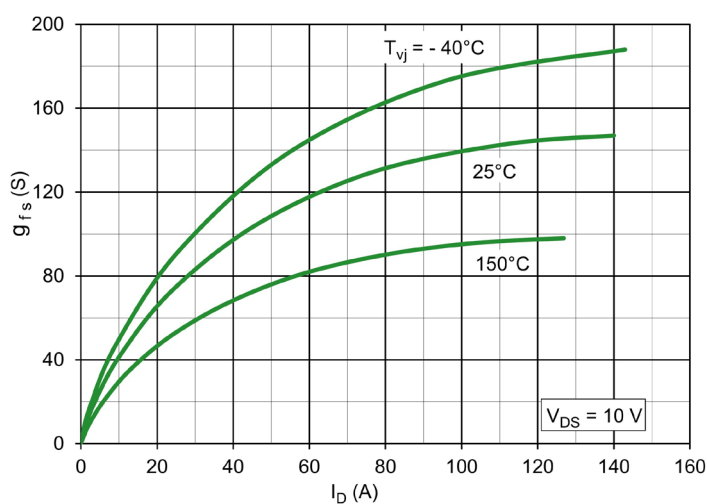
Figure 24. Typical Transconductance Curve
