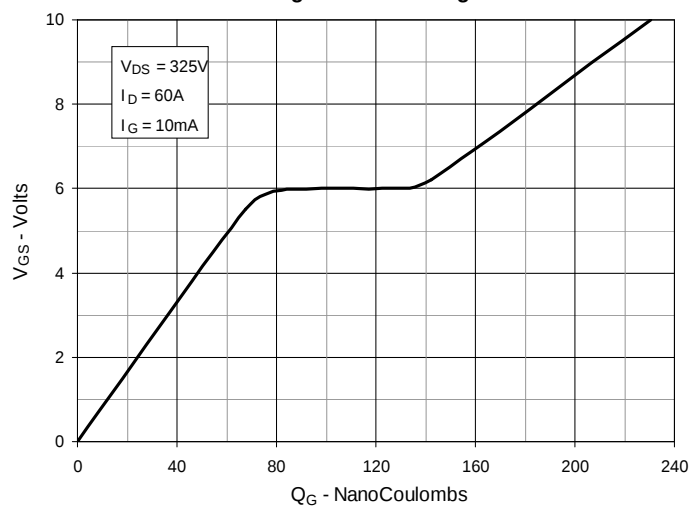
Fig. 11. Gate Charge
