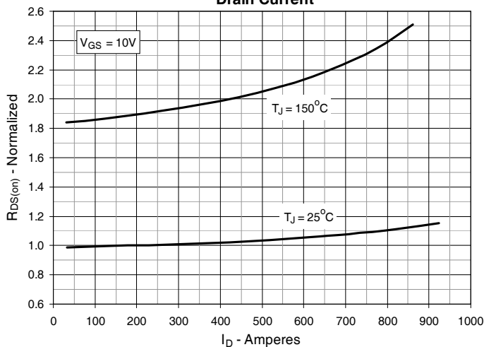
Fig. 5. R_{DS(on)} Normalized to I_D = 200A Value vs. Drain Current
