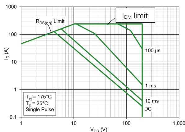
Figure 4. Forward-Bias Safe Operating Curve
