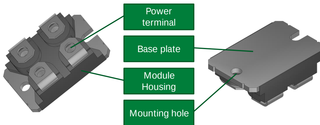
Figure 1: Littelfuse miniBLOC, in SOT227B
