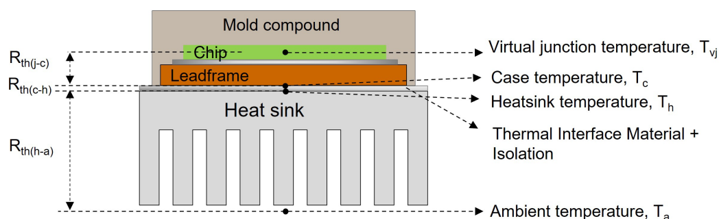
(a) Conventional Discrete Package
