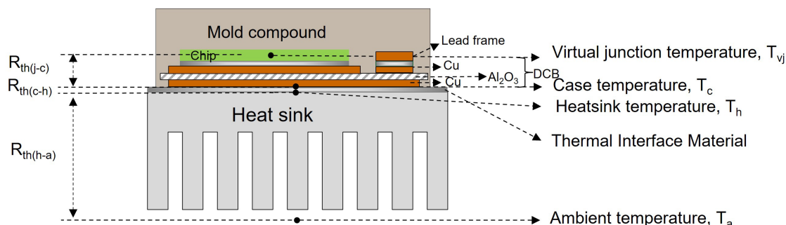
(b) Isolated Discrete Package
