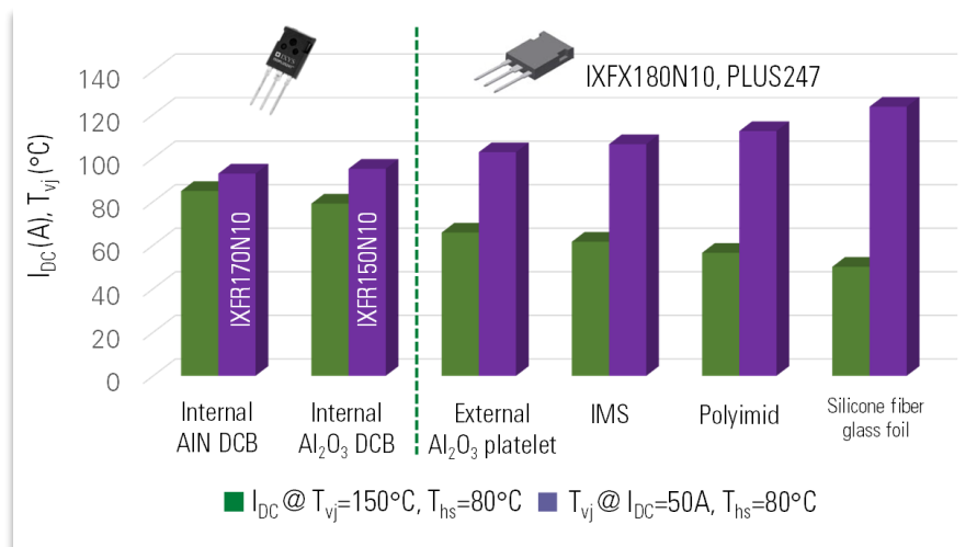
Figure 6. Comparing Electrical Performance of ISOPLUS™ 274 and PLUS247™ Devices
