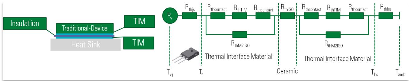
Figure 5. Thermal Model of a Non-insulated Package using a Ceramic Platelet and Thermal Grease
