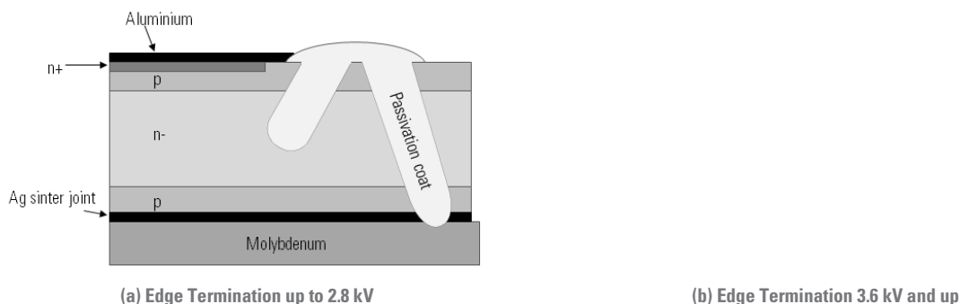
Figure 5. Detailed view to the Junction Terminations
