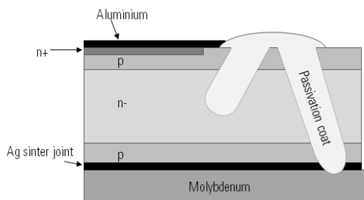
(a) Edge Termination up to 2.8 kV
