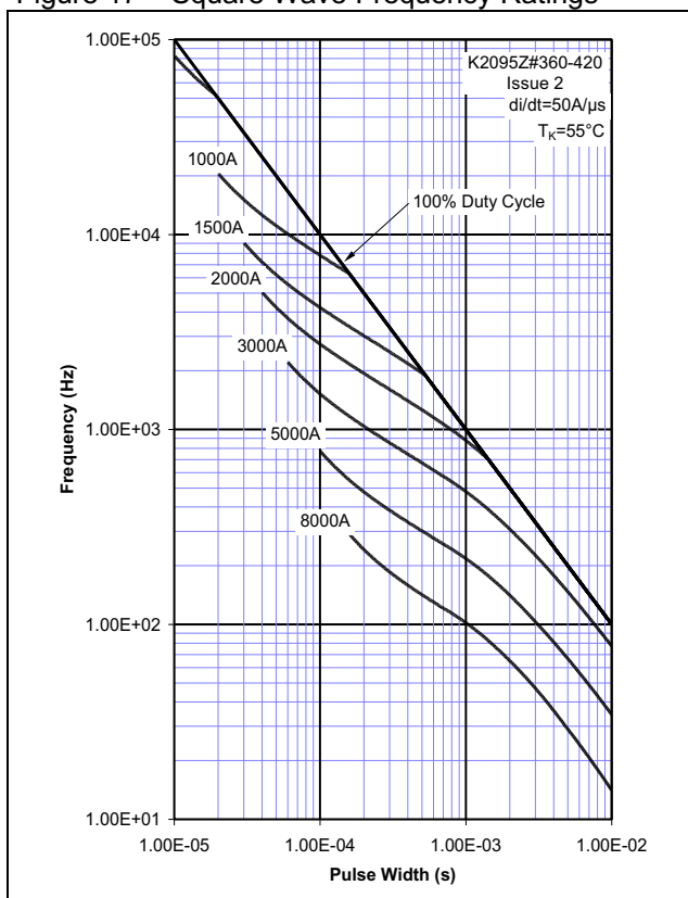
Figure 17 – Square Wave Frequency Ratings
