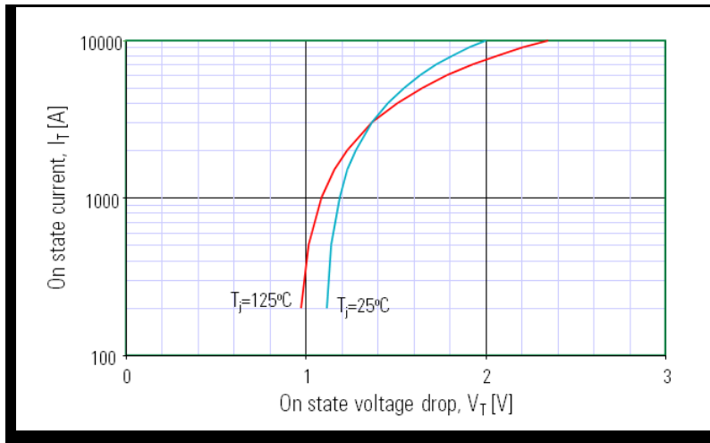
Figure 13. On-state Characteristic
