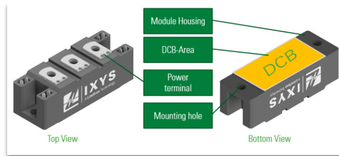
Figure 1. Littelfuse Y4-Package with Exposed DCB-Backside
