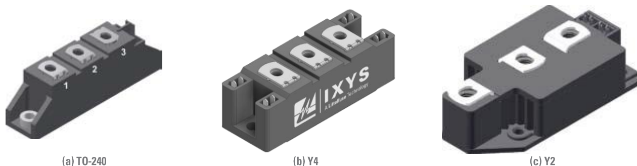
Figure 2. Package Illustration
