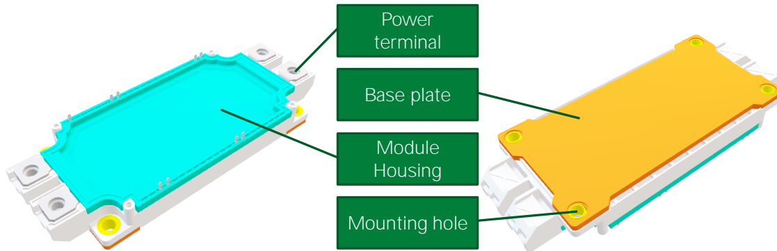
Figure 1: Littelfuse Simbus F Power Module, featuring a Solid Metal Base Plate
