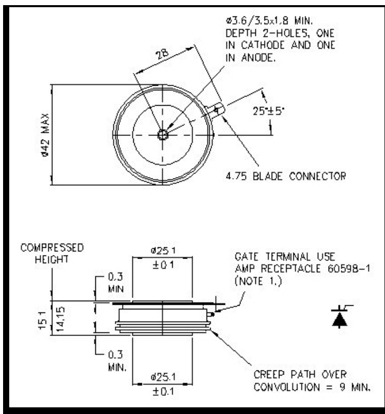
Figure 25. Typical Outline Drawing of a Capsule-type Thyristor
