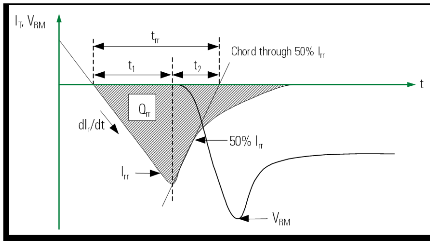
Figure 18. Reverse Recovery Characteristics
