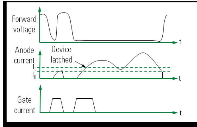
Figure 15. Correlation between Holding Current and Latching Current
