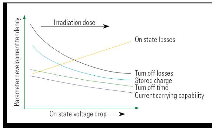
Figure 4. Impact of Irradiation Dose to the Device's Parameters
