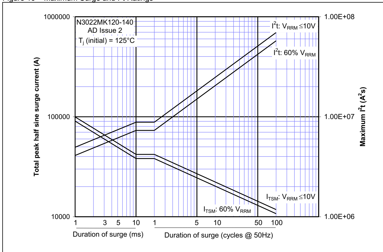
Figure 16 – Maximum Surge and I^2t Ratings
