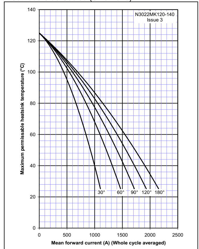
Figure 13 – On-state current vs. Heatsink temperature – Cathode Side Cooled (Sine wave)
