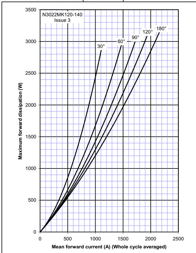
Figure 12 – On-state current vs. Power dissipation – Cathode Side Cooled (Sine wave)
