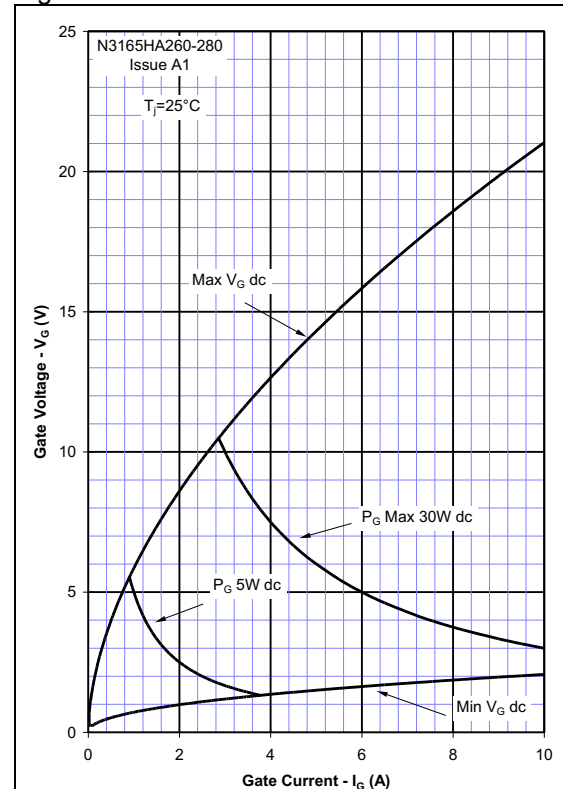
Figure 4 - Gate Characteristics - Power Curves
