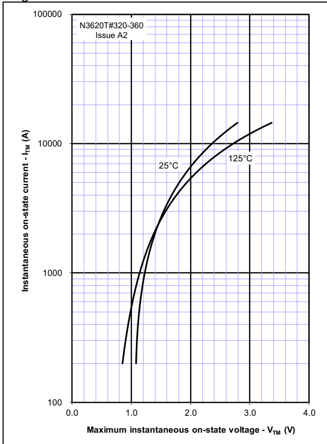
Figure 1 – On-state characteristics of Limit device
