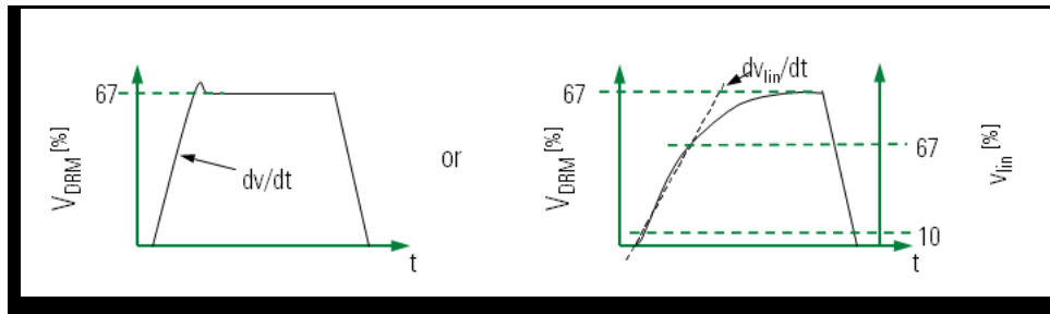
Figure 14. Approximations for dv/dt_{(crit)}
