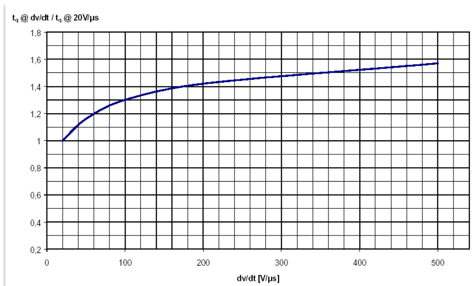
Figure 21. Dependency of t_q on Voltage Change Rate dv/dt , normalized to 20V/ \mu s
