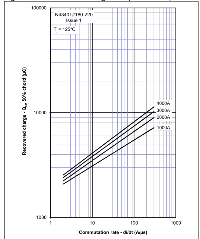
Figure 6 – Recovered Charge, Q_{ra} (50% chord)
