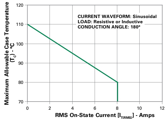
Figure 4: Maximum Allowable Case Temperature vs. RMS On-State Current
