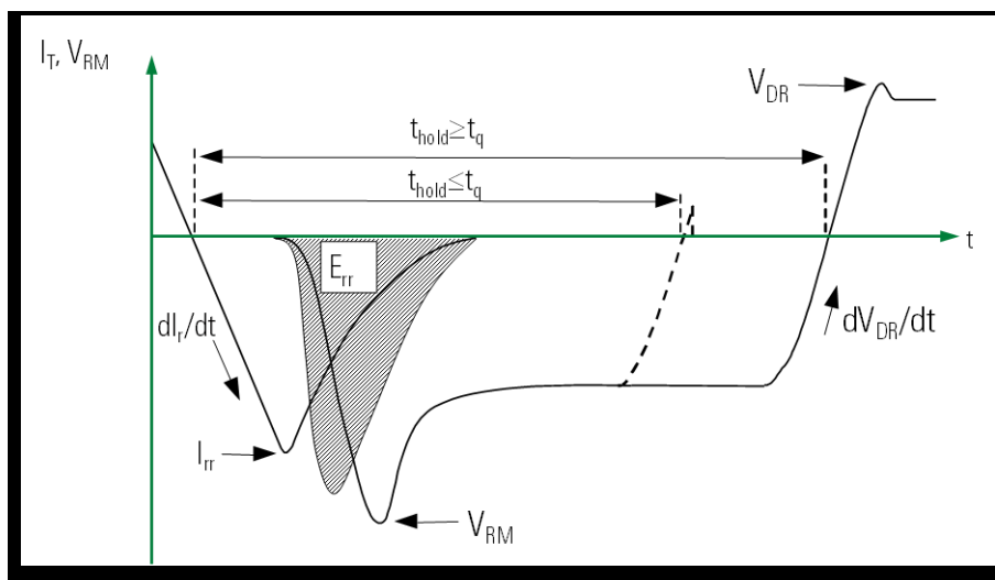
Figure 19. Circuit Commutated Turn-off Time
