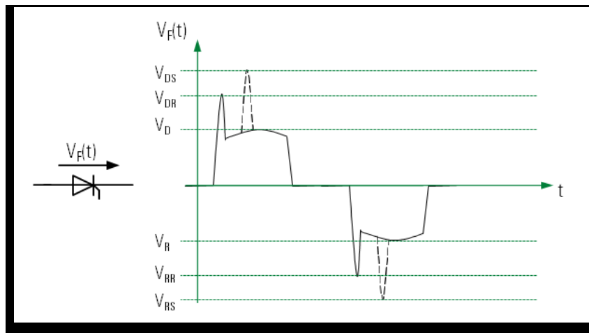
Figure 9. Typical Voltage Waveforms
