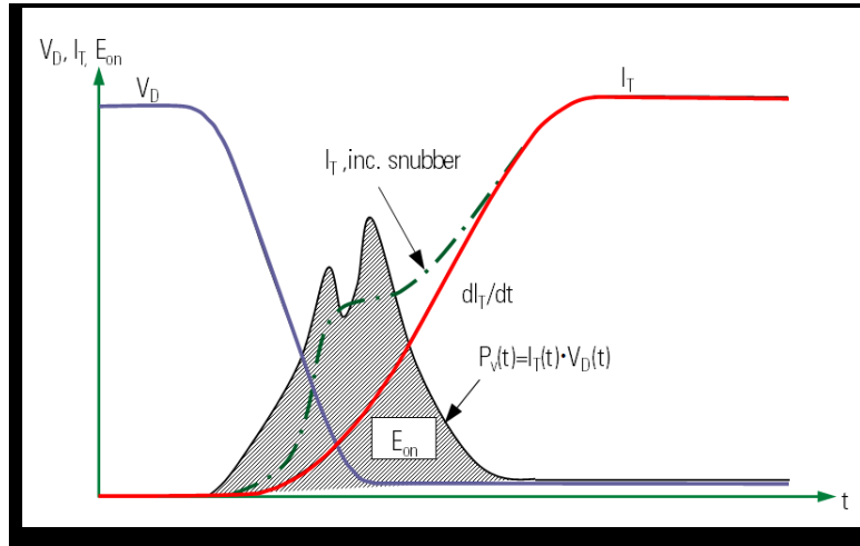
Figure 17. Turn-on Energy
