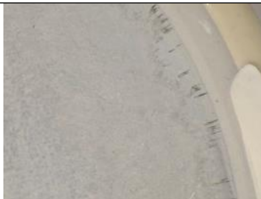
Figure 2: Initial evidence of thermal cycling scrubbing at the edge on the cathode contact area
