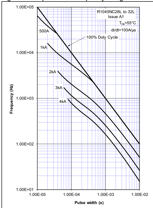
Figure 13 - Square wave frequency ratings
