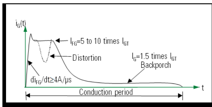
Figure 12. Gate-Current Waveform
