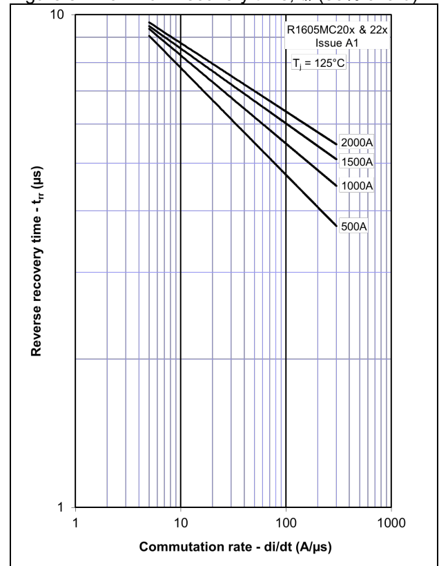
Figure 8 - Maximum recovery time, t_{rr} (50% chord) (μs)
