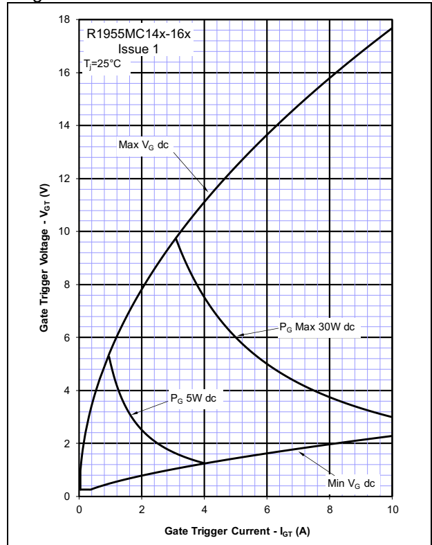
Figure 4 - Gate characteristics - Power curves
