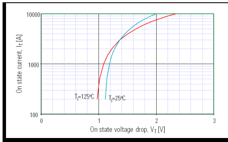
Figure 13. On-state Characteristic
