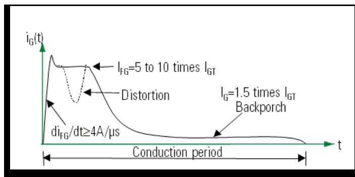
Figure 12. Gate-Current Waveform
