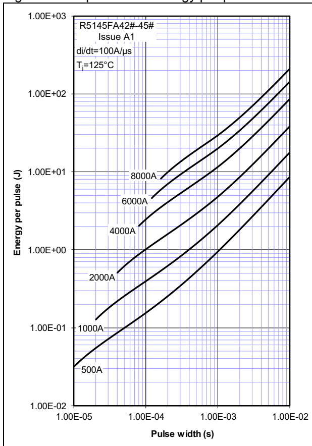
Figure 17 - Square wave energy per pulse
