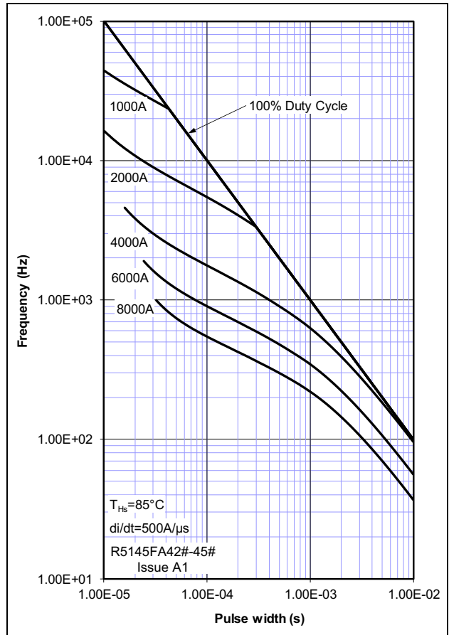
Figure 16 - Square wave frequency ratings
